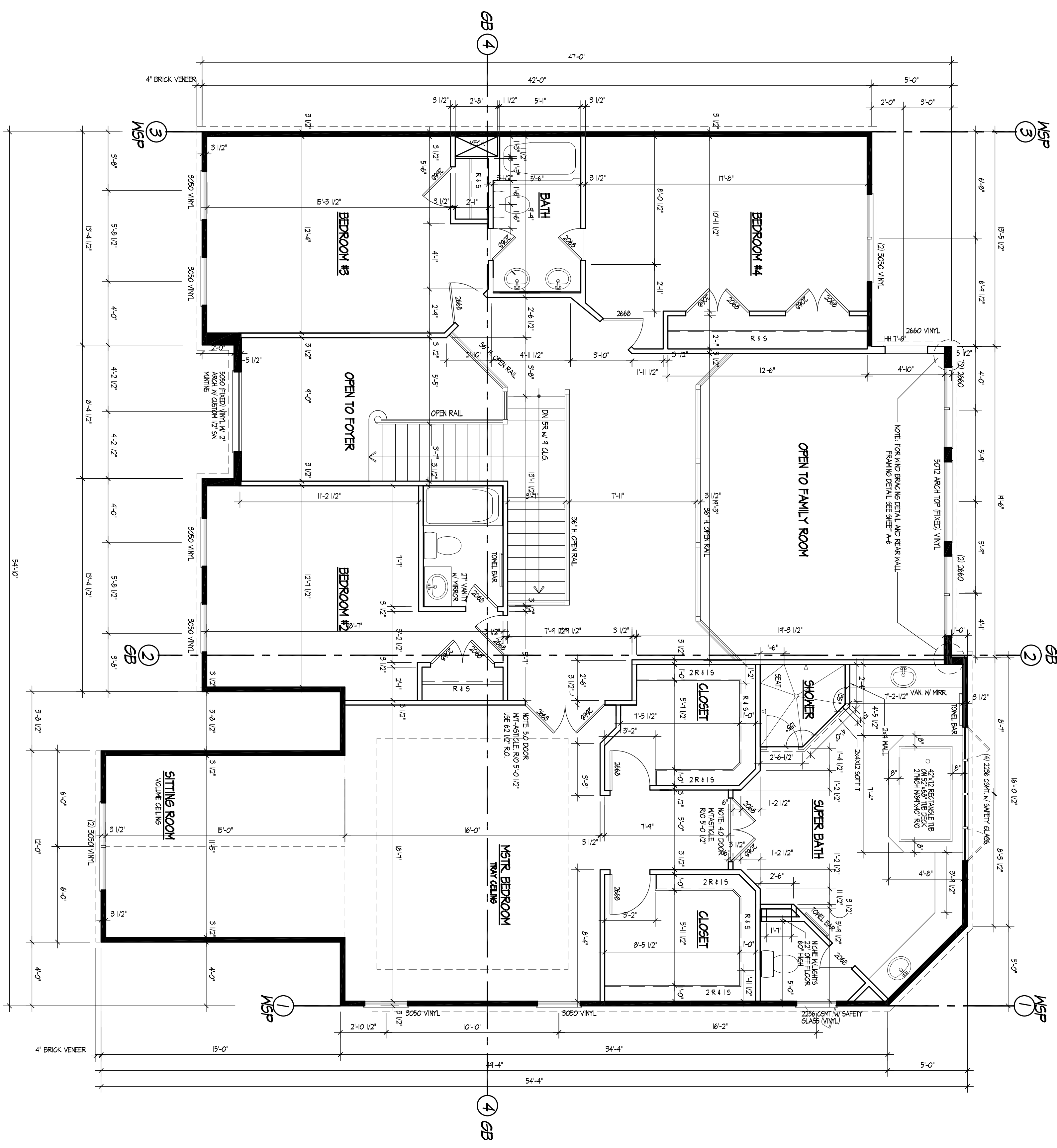
SECOND FLOOR PLAN SCALE 1/8" = 1'-0"
